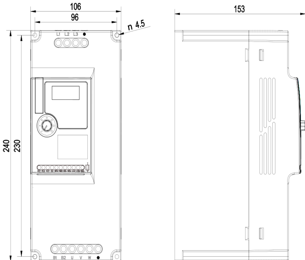
Dimensional drawing A550 Plus - 11kW 4T0110
