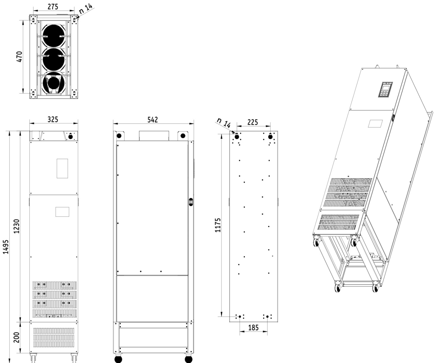
Dimensional drawing V900 - 355kW 4T3550
