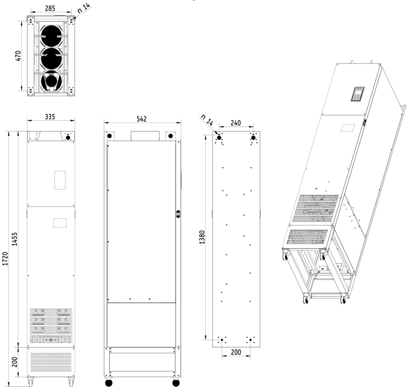
Dimensional drawing V900 - 400kW 4T4000
