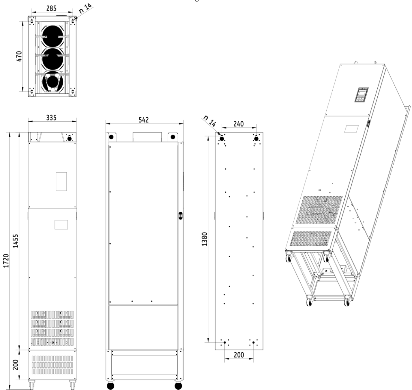
Dimensional drawing V900 - 450kW 4T4500
